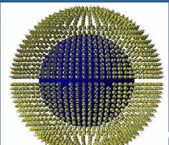
Courtesy Borexino
